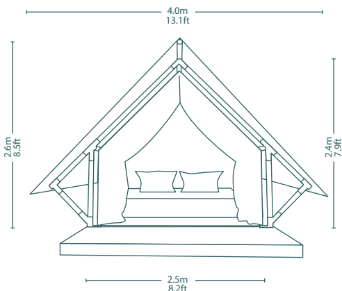
Etched aluminum framework and steel connectors
