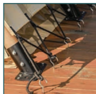
Reinforcement tightening
